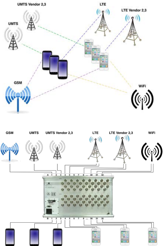
(fig. 6. Handover test setup)
